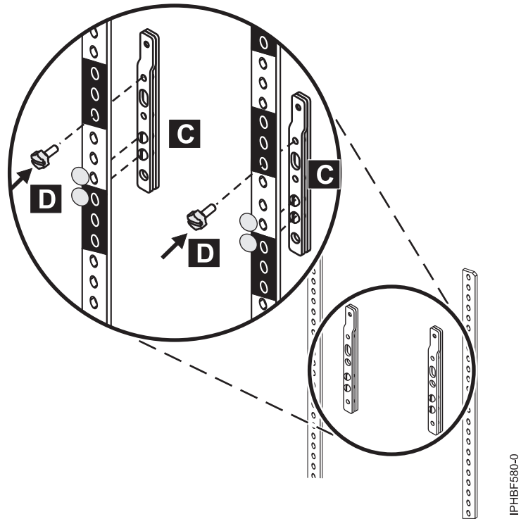
Figure 47. Attaching the front rail-mount bracket
