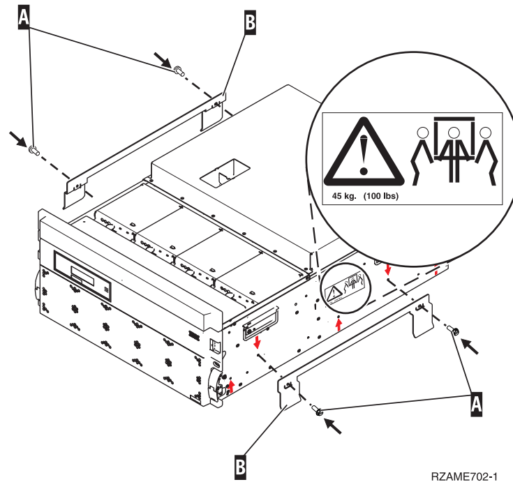
Figure 50. Attaching the rail-mounting guides
