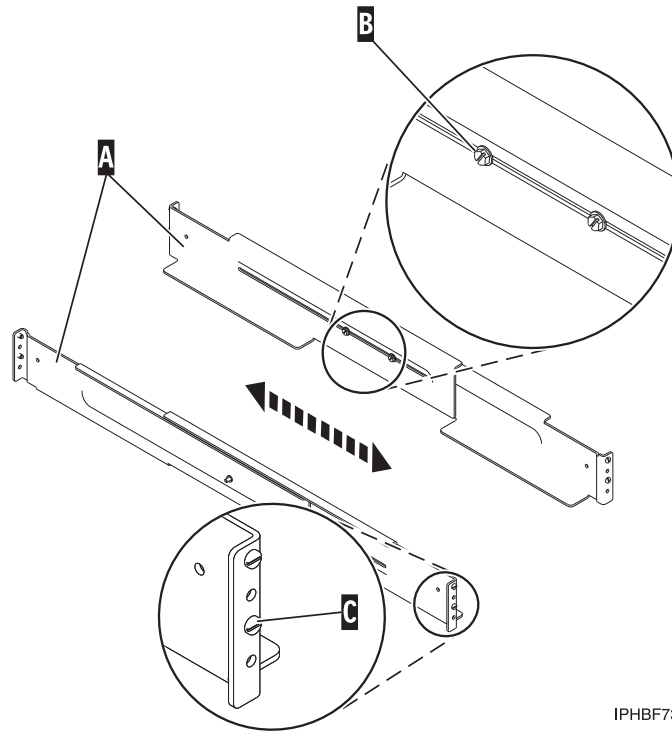
Figure 99. Extending the system rails
