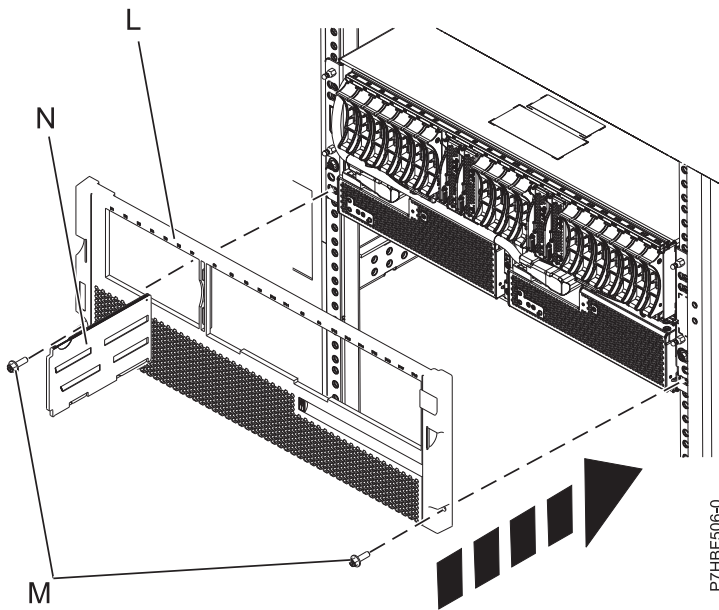
Figure 64. Installing the bezel and service information holder
