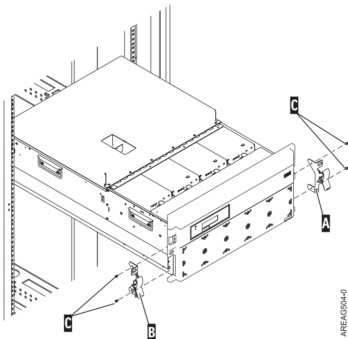
Figure 124. Removing the retaining screws
