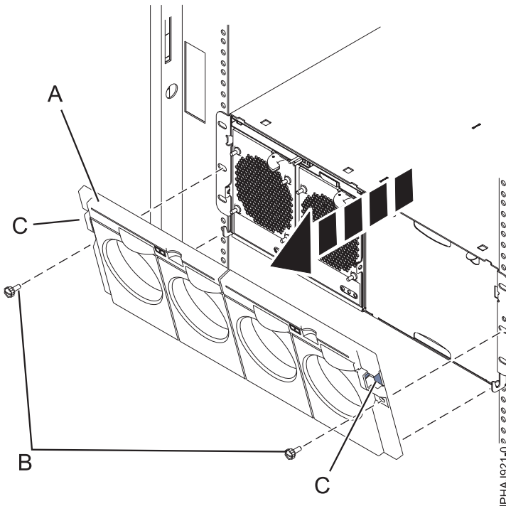
Figure 131. Remove the front cover for model 7314-G30 or 5796
