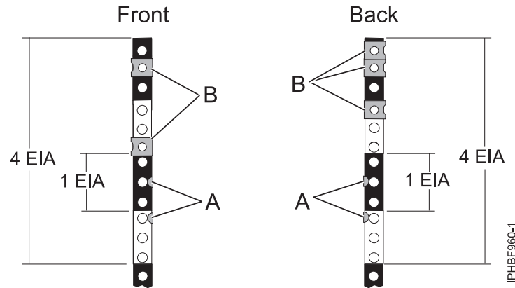
Figure 81. EIA units with the expandable rails for the 5790 drawer
