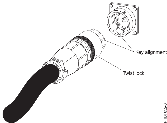
Figure 130. Aligning the connector on the power cord with the PDU+.
