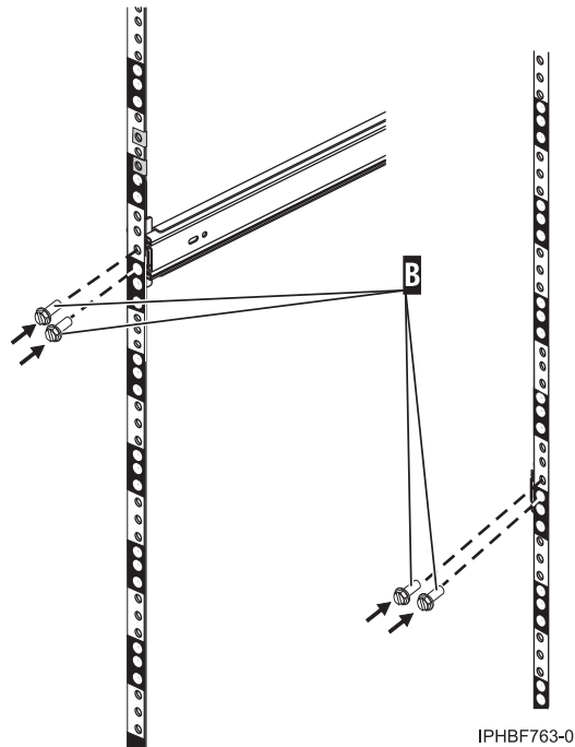
Figure 46. Attaching the rails to the back of the rack
