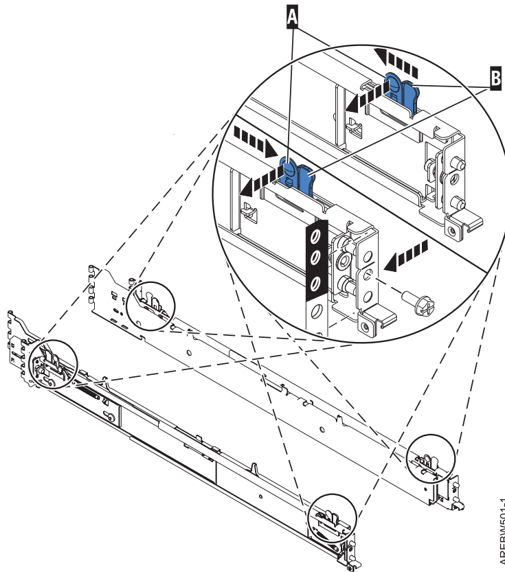
Figure 22. Front slide rail alignment pin, retaining screws, and latch bracket
