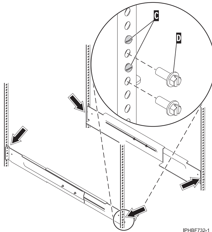
Figure 100. Attaching the system rails
