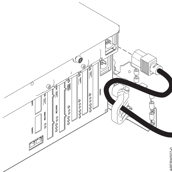
Figure 42. Routing server power cord
