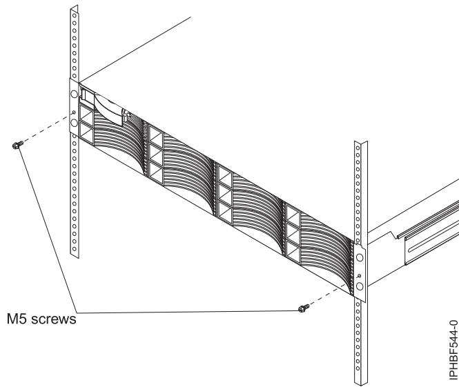
Figure 73. Installing the securing screws
