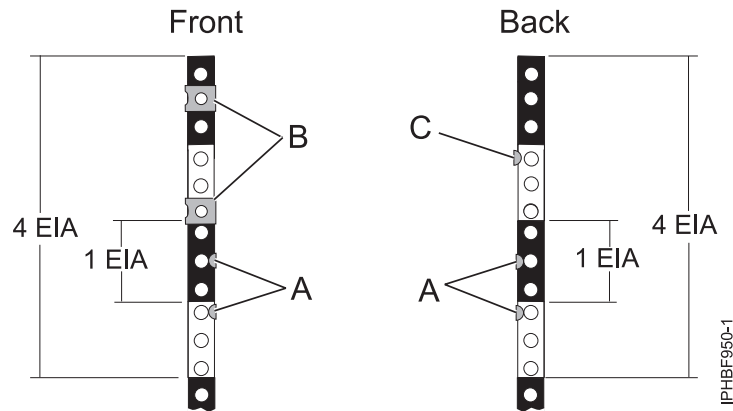
Figure 82. EIA units with the expandable rails for the 5796 drawer
