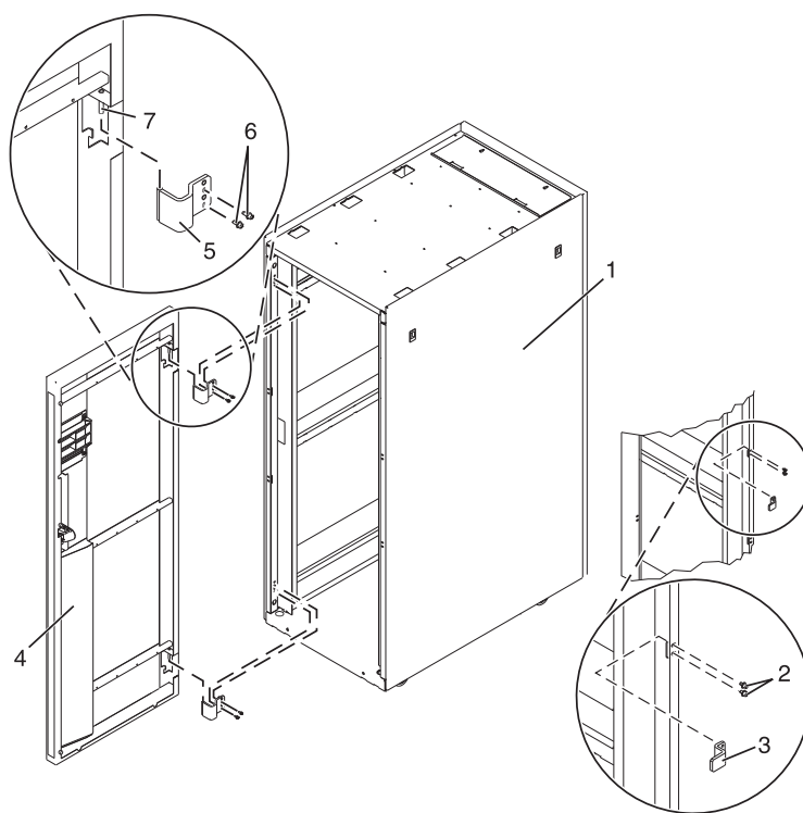
Figure 108. Attaching the rack door
