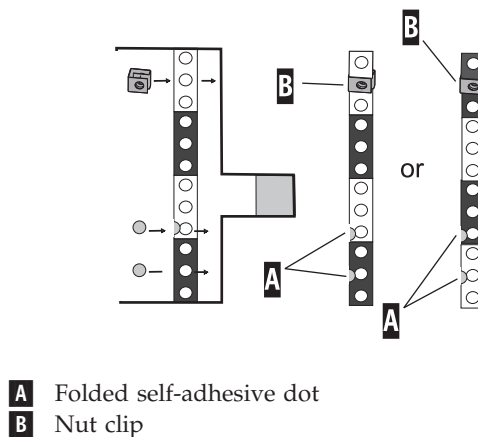
Figure 79. Attaching the dots and nut clips for the standard rails
