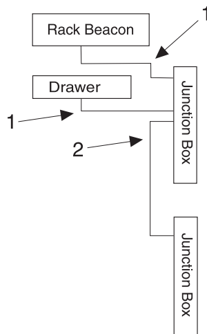
Figure 120. Connecting the rack status beacon and system unit to the junction box
