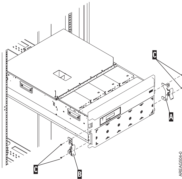
Figure 123. Reinstalling the latch brackets
