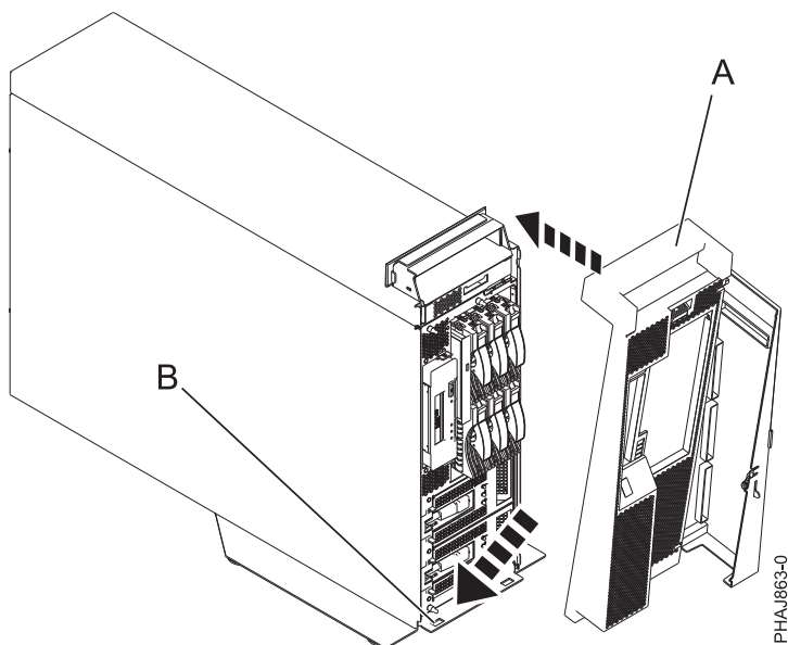
Figure 141. Replacing the cover on the model
