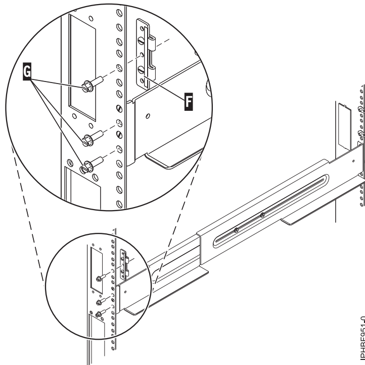
Figure 87. Attaching the rails to the back of the rack
