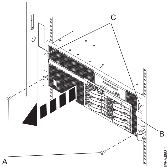
Figure 138. Removing the front cover from a rack-mounted model
