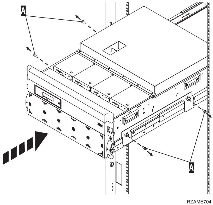
Figure 52. Removing the rail-mounting guides
