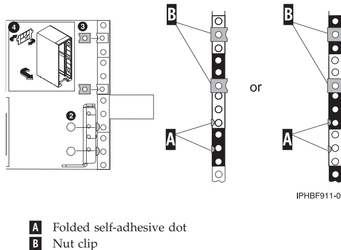
Figure 80. Attaching the dots and nut clips for the expandable rails
