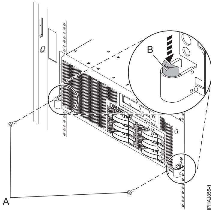
Figure 149. Releasing the rack latches
