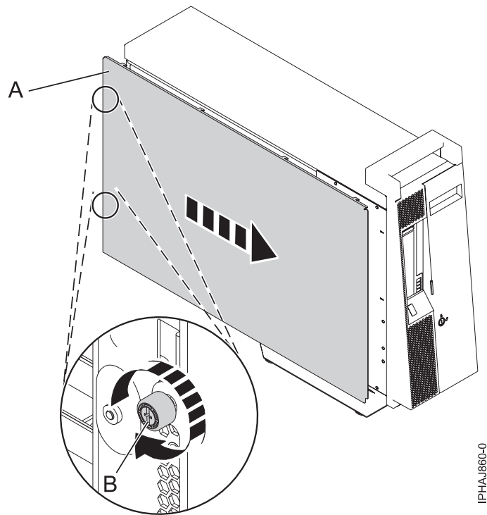
Figure 137. Installing the service access cover on a stand-alone model
