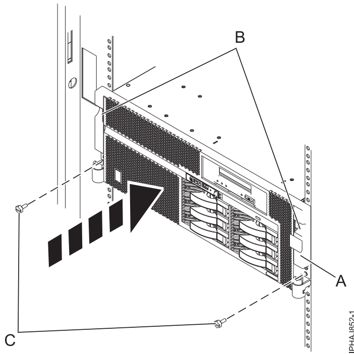
Figure 148. Pushing the system into the rack and attaching the thumbscrews
