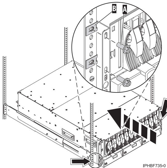
Figure 102. Installing the securing screws.
