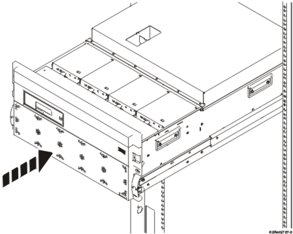
Figure 55. Sliding the expansion unit into the rack
