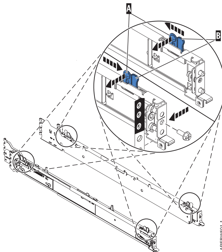
Figure 36. Front slide rail alignment pin
