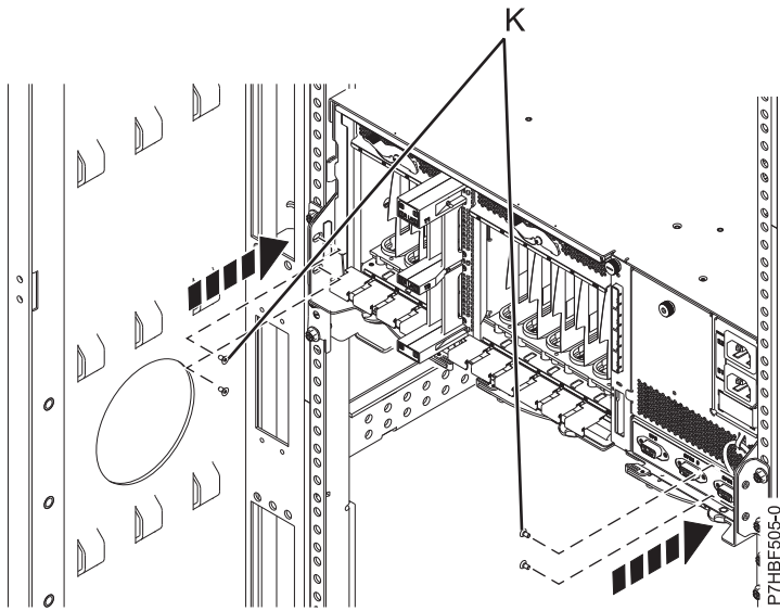
Figure 63. Sliding the expansion unit in the rack
