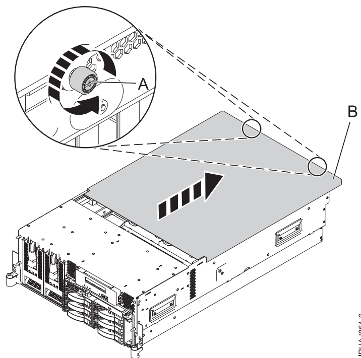
Figure 134. Remove the service access cover from a rack-mounted model
