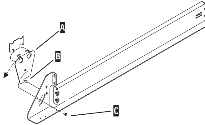
Figure 105. Rotating the cable-management arm
