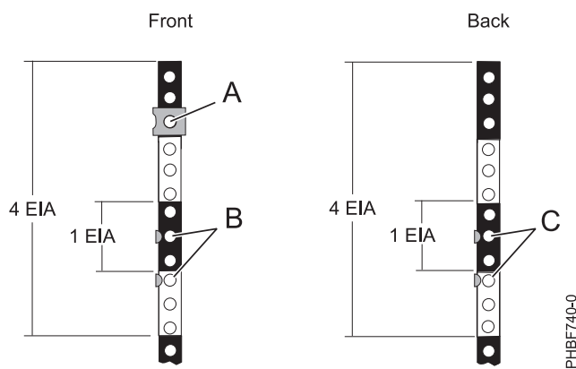
Figure 57. Marking the installation locations
