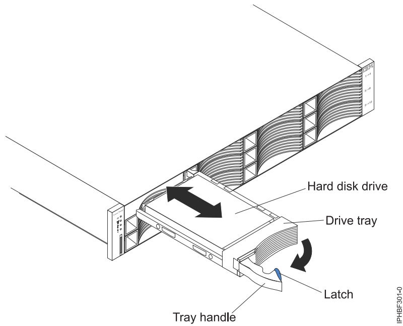
Figure 72. Removing disk drives
