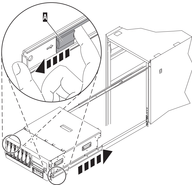
Figure 147. Releasing the rail safety latches
