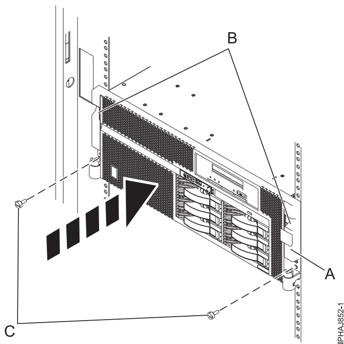
Figure 151. Replacing the thumbscrews
