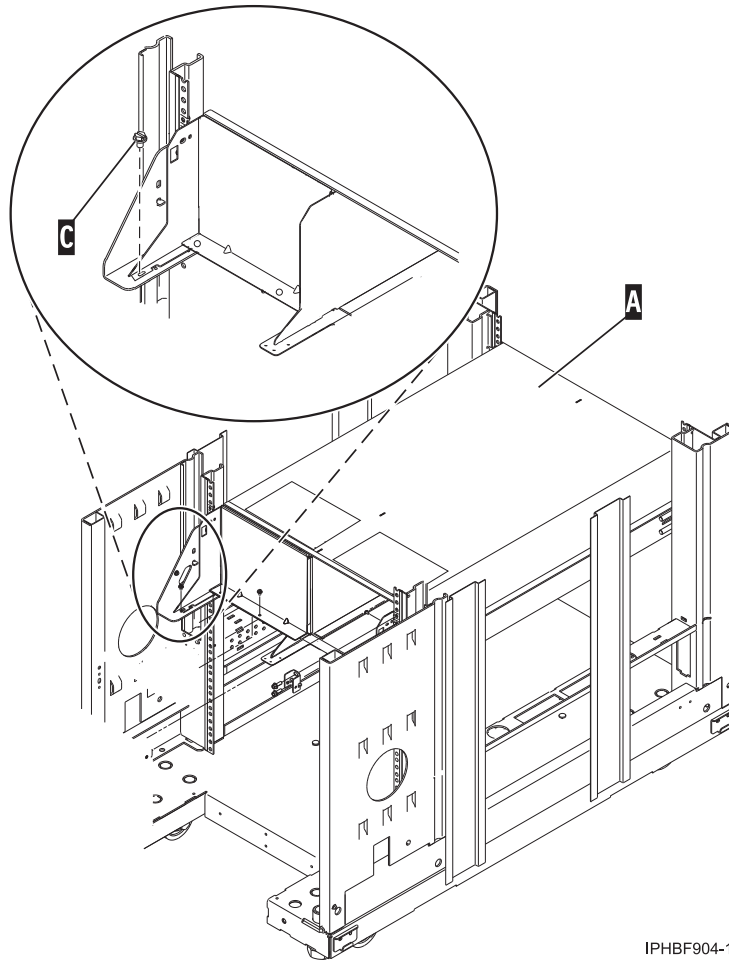
Figure 90. Securing the shell to the rack with the expandable rails
