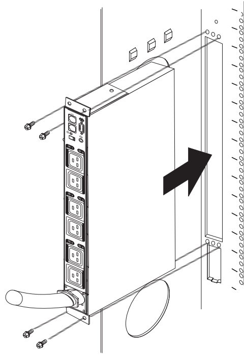
Figure 126. Aligning the PDU+ with the opening in the side of the rack
