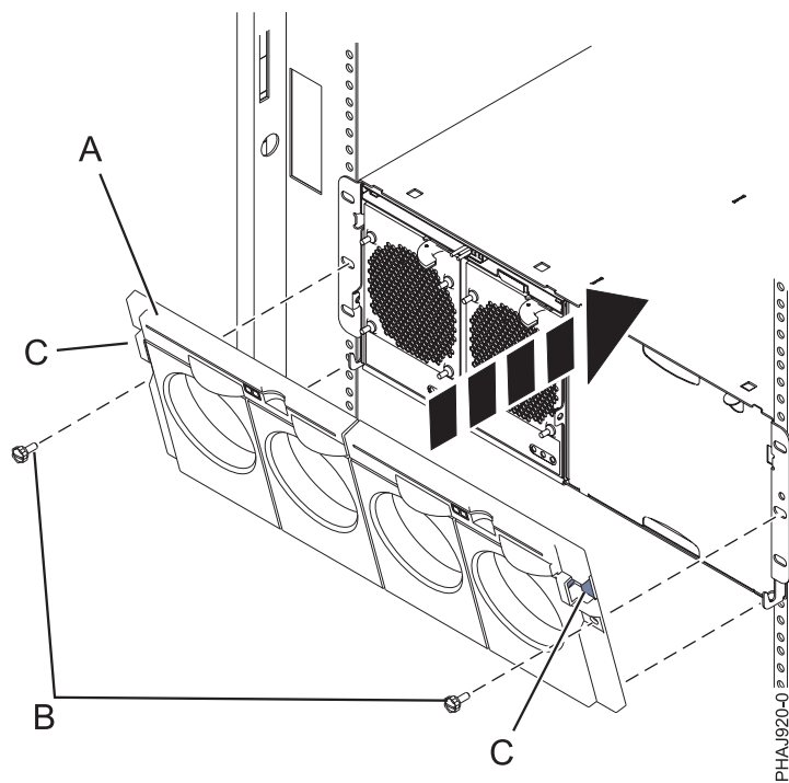
Figure 132. Front cover on a model 7314-G30 or 5796
