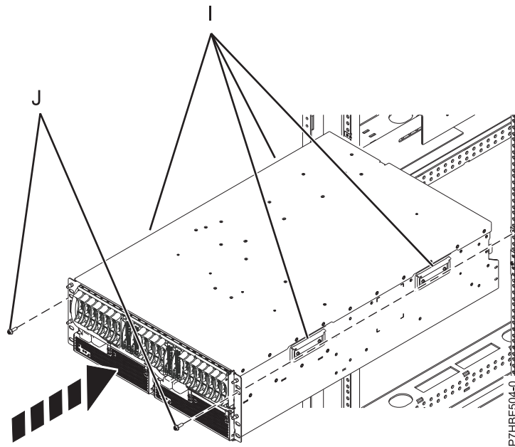
Figure 62. Installing the expansion unit into a rack
