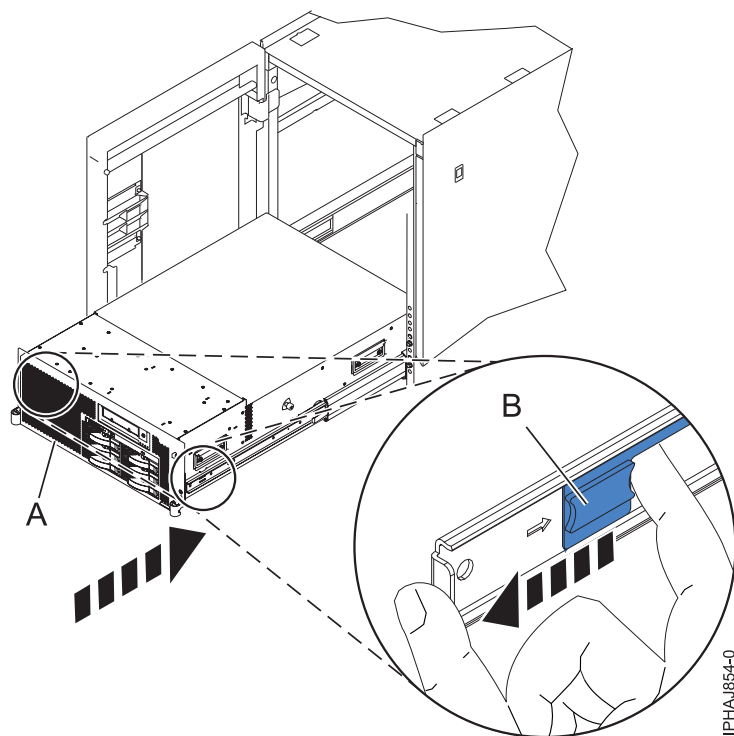
Figure 150. Releasing the rail safety latches
