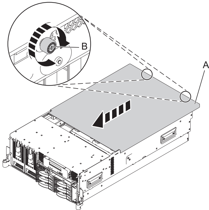
Figure 135. Install the service access cover on the rack-mounted model
