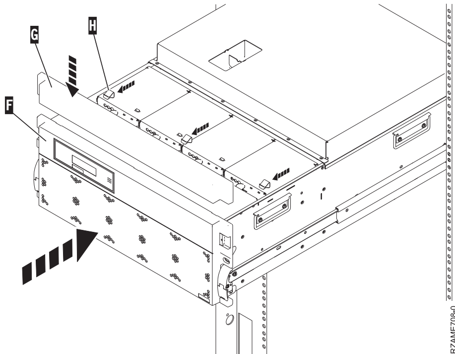
Figure 49. Installing the cover attachment to the cover
