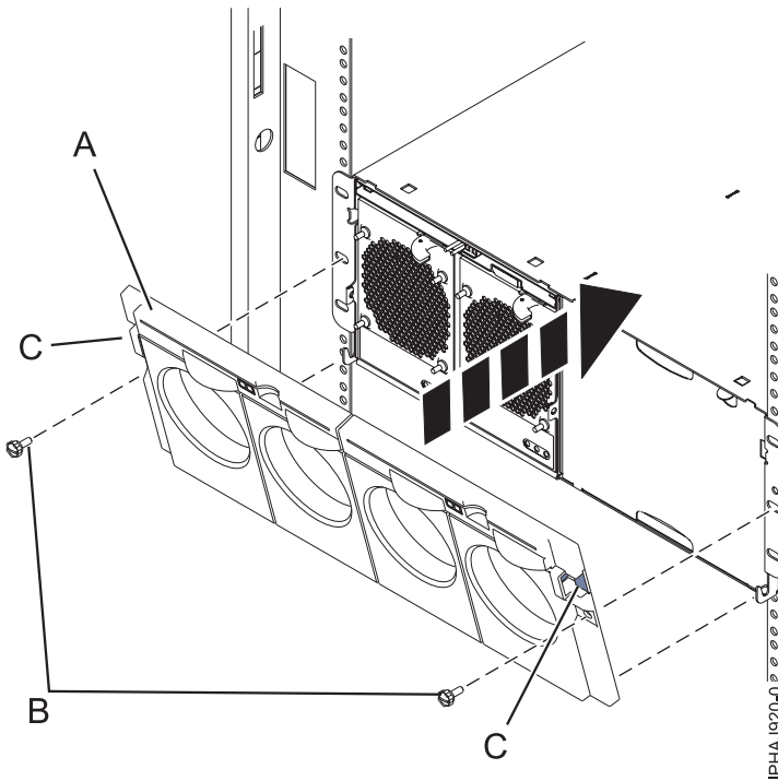
Figure 142. Front cover on a model 7314-G30 or 5796
