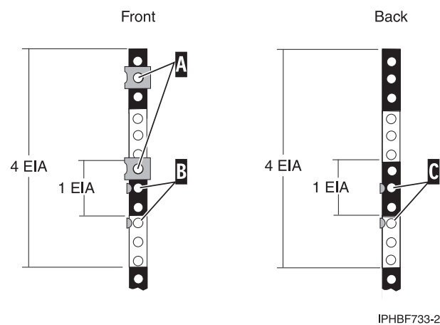
Figure 96. Marking the installation locations
