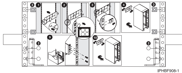
Figure 74. Rack-mounting template for the expandable rails
