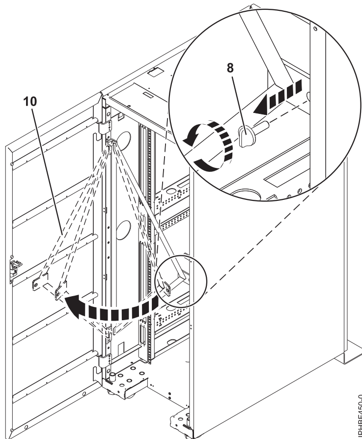
Figure 115. Releasing the brace to access systems
