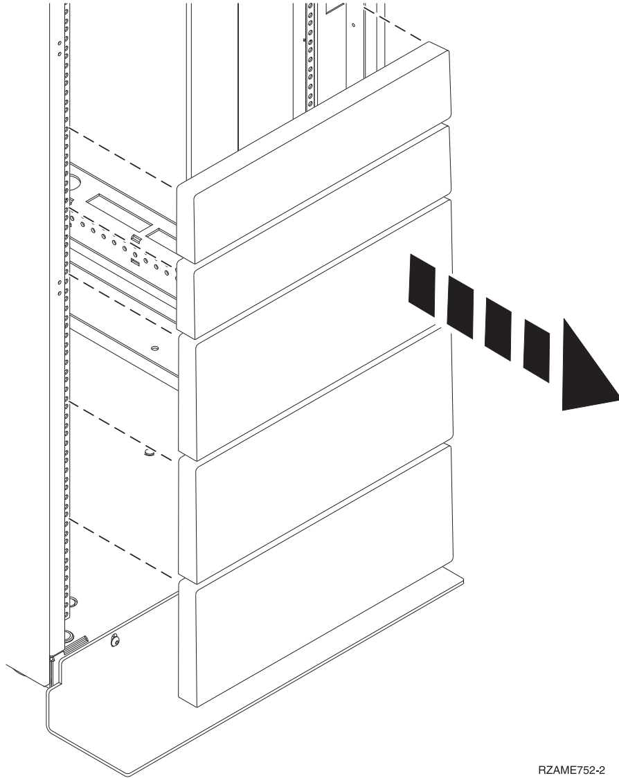
Figure 95. Removing the filler panels
