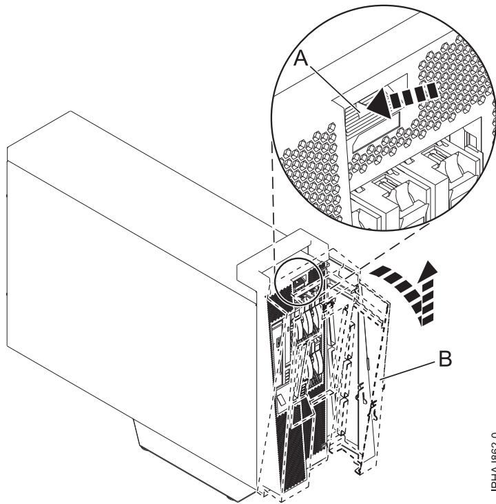
Figure 140. Remove the door from the model
