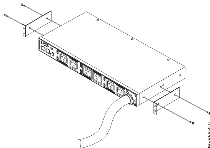
Figure 128. Aligning the vertical-mounting brackets to the front of the PDU+.
