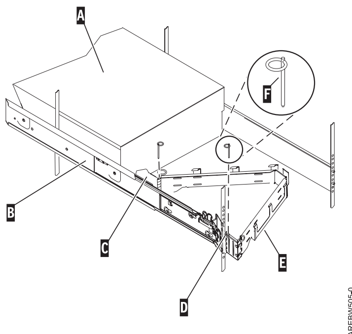
Figure 41. Attaching the cable-management arm
