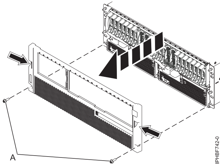
Figure 61. Removing the service information holder and bezel
