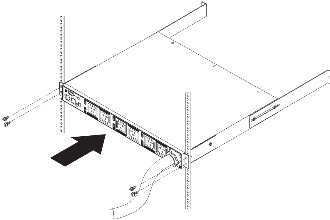
Figure 129. Aligning the PDU+ with the opening in the rack.
