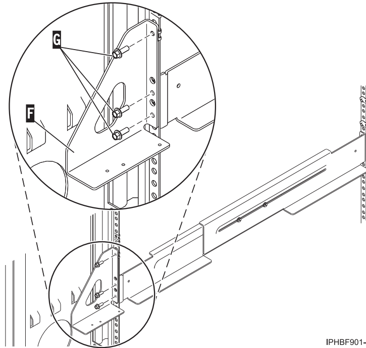
Figure 86. Attaching the extension brackets and rails to the back of the rack
