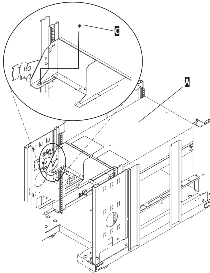
Figure 89. Securing the shell to the rack with the standard rails
