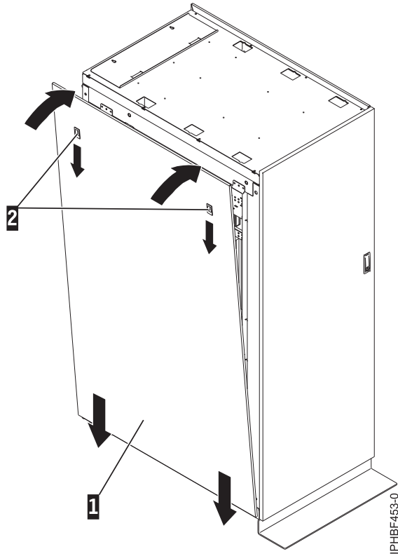
Figure 107. Replacing the side panel
