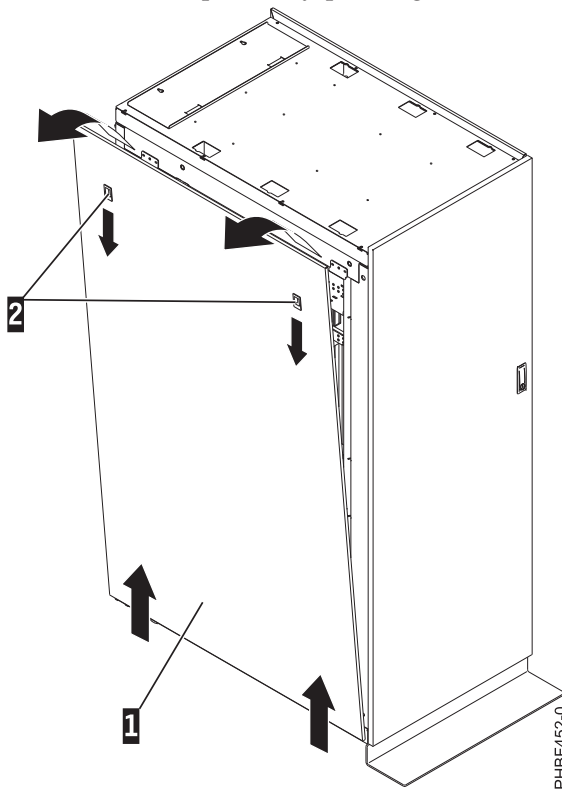
Figure 106. Removing the side panel
