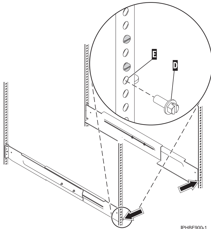
Figure 85. Attaching the system rails to the front of the rack
