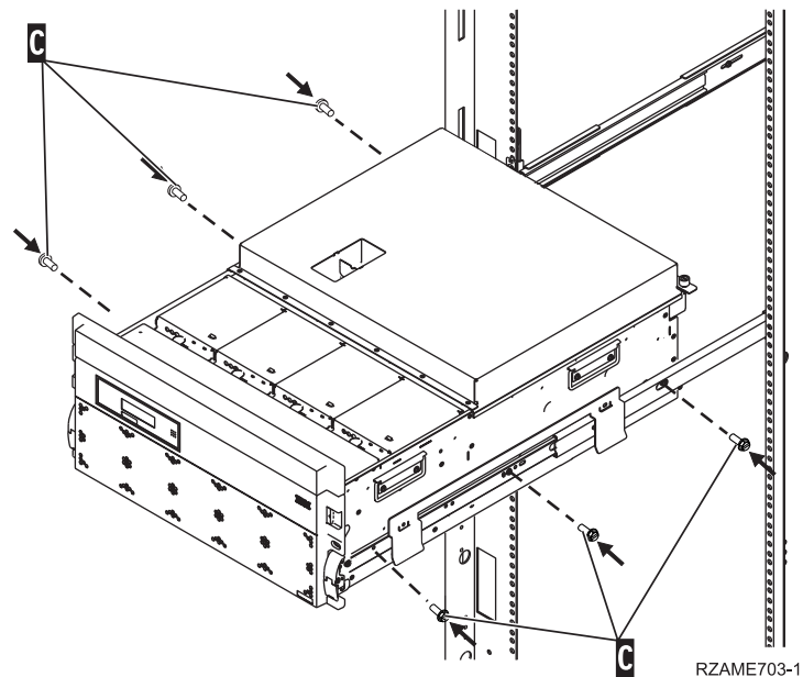
Figure 51. Installing the expansion unit onto the rails
