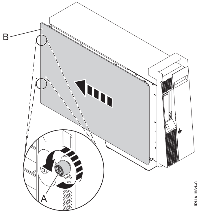
Figure 136. Removing the service access cover from the stand-alone model
