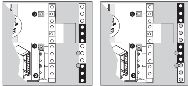
Figure 97. Example of a rack-mounting template
