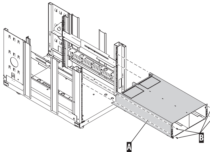
Figure 88. Installing the shell into the rack on the expandable rails
