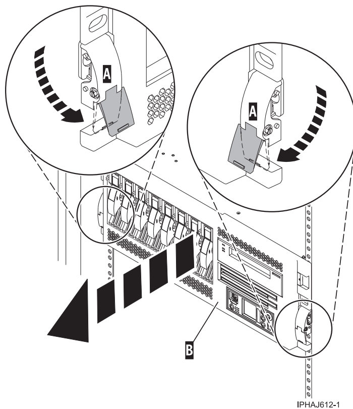
Figure 146. Releasing the rack latches
