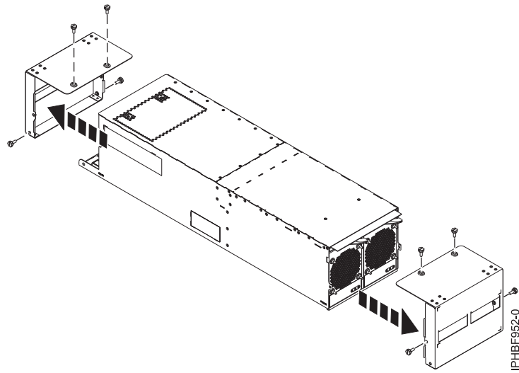
Figure 91. Removing the shipping covers
