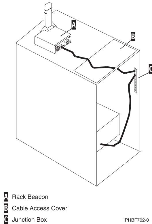
Figure 119. Connecting the rack status beacon to the system unit through the junction box
